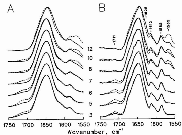
FIGURE 2 Infrared amide I band region of the original (A) and deconvoluted (B) spectra of the ShB (—) and the ShB-L7E (---) peptides in D_2O media prepared from 10 mM phosphate buffers at the indicated pH values (3–12), containing 130 mM KCl and 20 mM NaCl.
