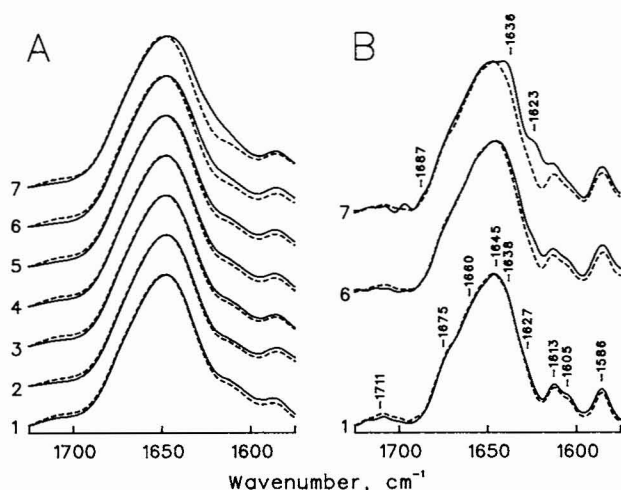
FIGURE 1 Infrared amide I band region of the original (A) and deconvoluted (B) spectra of the ShB (—) and the ShB-L7E (---) peptides in plain D_2O (traces 1) or in different D_2O media prepared from 10 mM HEPES, pH 7.4 (traces 2); 5 mM HEPES, pH 7.0, containing 130 mM KCl, 20 mM NaCl (traces 3); 5 mM HEPES, pH 7.0, containing 2 mM CaCl_2 , 115 mM NaCl, 2 mM KCl (traces 4); or 10 mM HEPES, pH 7.4, containing 100 mM (traces 5), 200 mM (traces 6), or 300 mM NaNO_3 (traces 7). In this and in all other figures, the spectra of the different buffers alone were subtracted from those of the peptide-containing samples. Numbers on top of the spectra in B and in all other figures represent the wavenumbers of the most characteristic components detected upon deconvolution. Temperature was maintained at 20°C.
